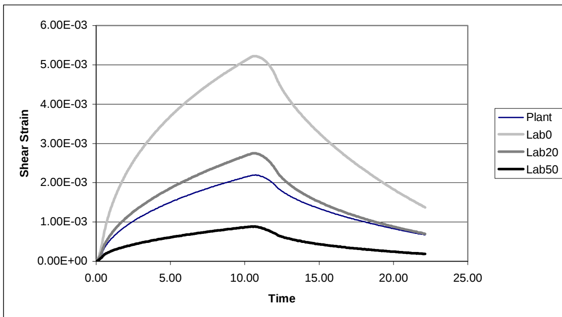
Figure 23 Average Shear Strains for Missouri Mixes at 40°C
