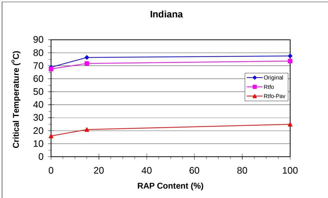
Figure 1 Critical Temperatures vs. RAP Content - Indiana
