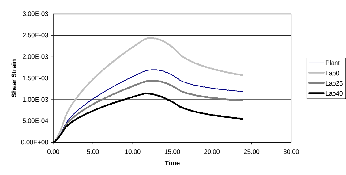
Figure 20 Average Shear Strains for Michigan Mixes at 20°C
