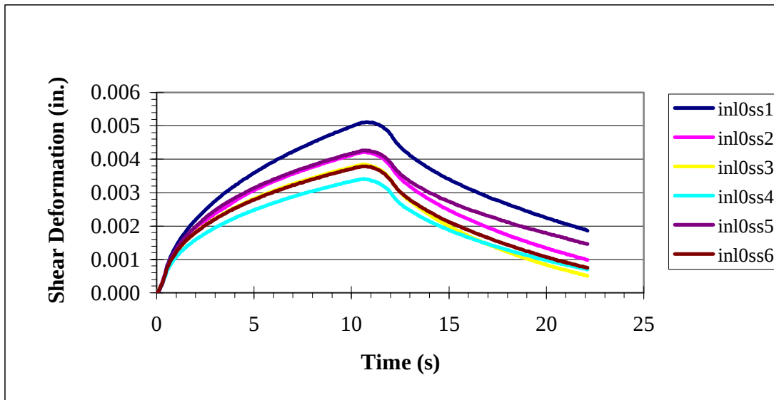
Figure 19 Examples Showing Typical Variability in Replicate Test Results
