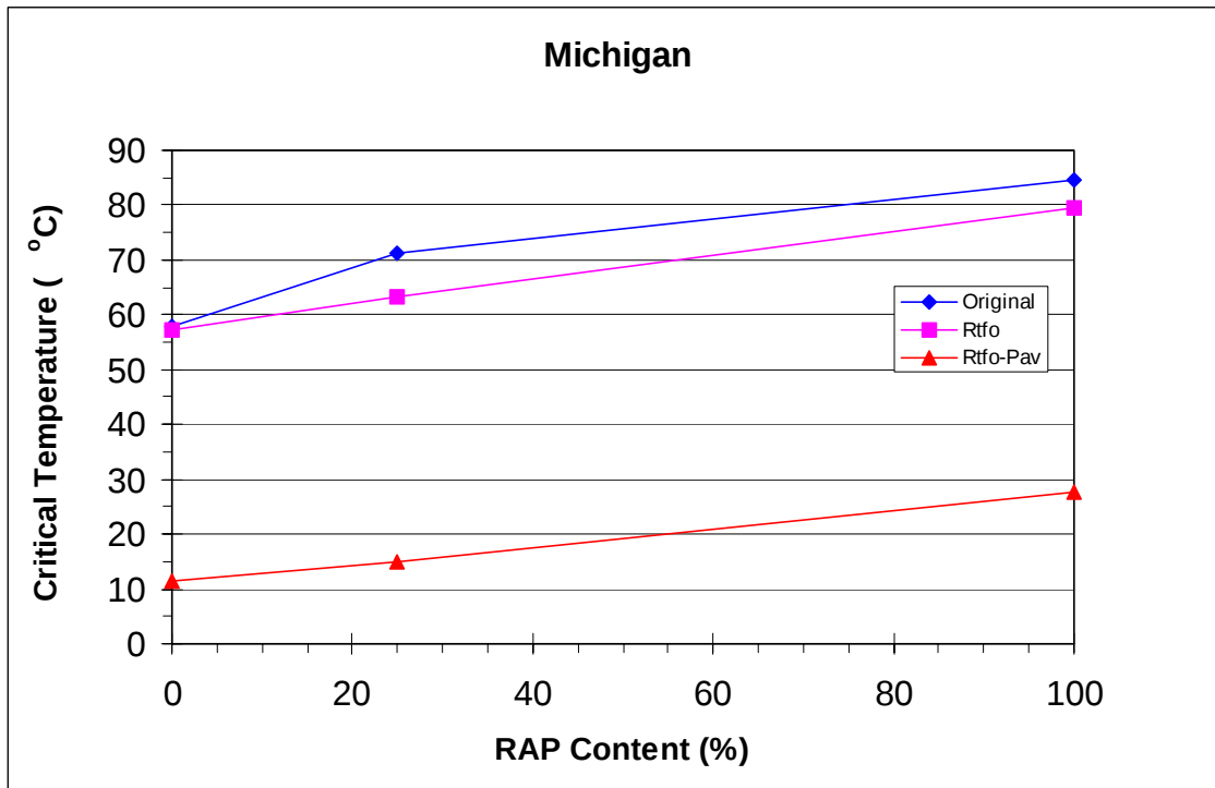
Figure 2 Critical Temperatures vs. RAP Content - Michigan
