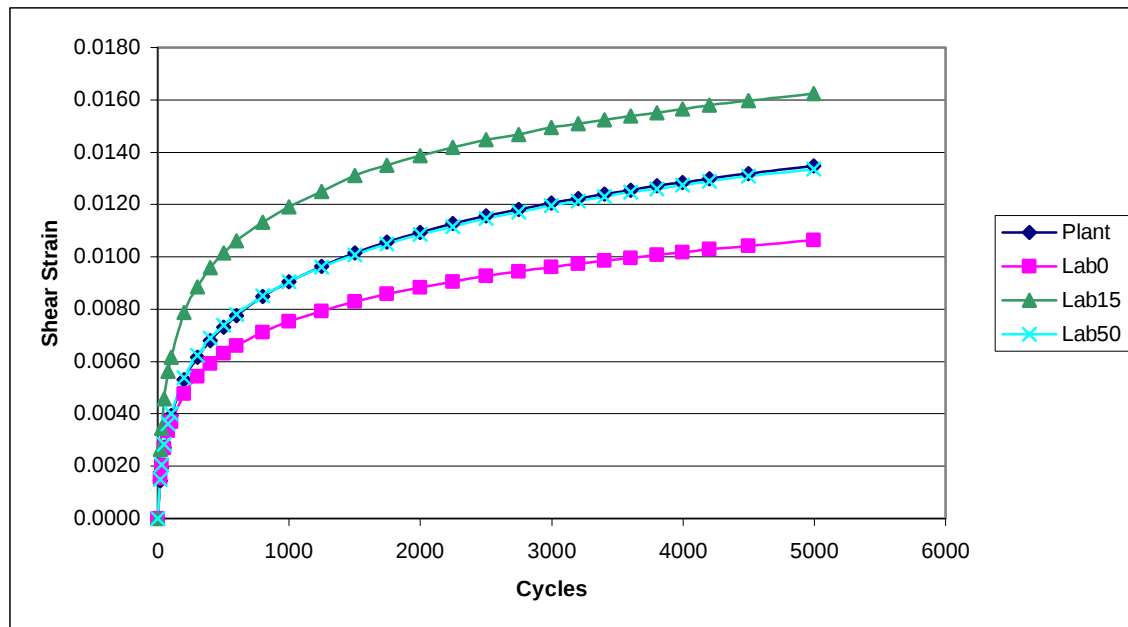
Figure 24 Average Shear Strain from RSCH Test, Indiana Mixes
