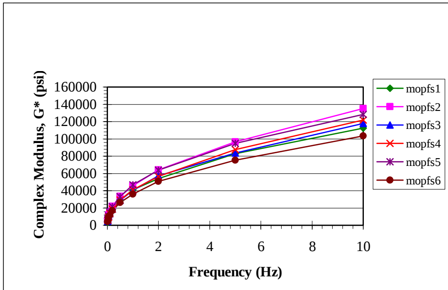
Figure 4 Frequency Sweep Results for Missouri Plant Mix Replicates (40°C)
