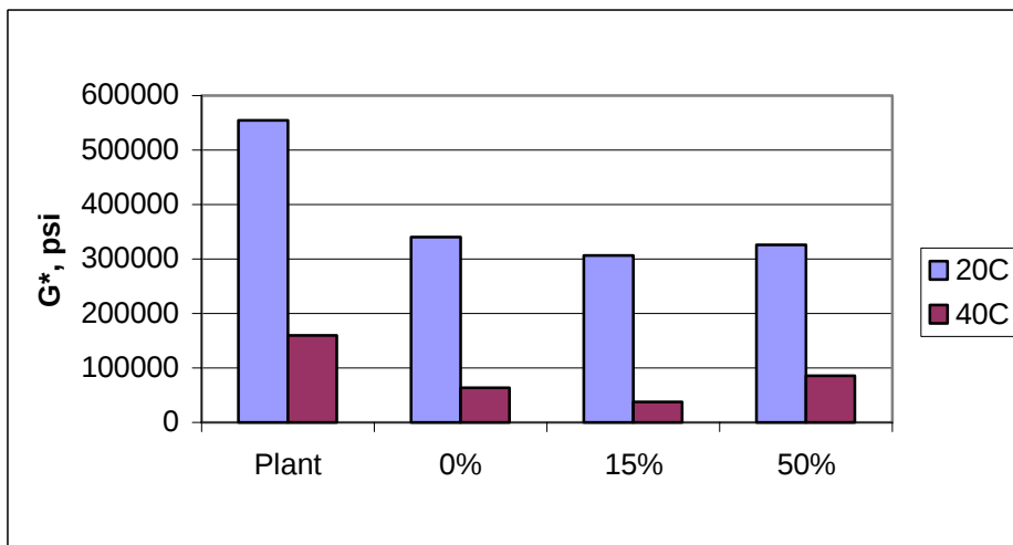
Figure 10 Summary of Complex Shear Moduli from Frequency Sweep at 10 Hz, Indiana
