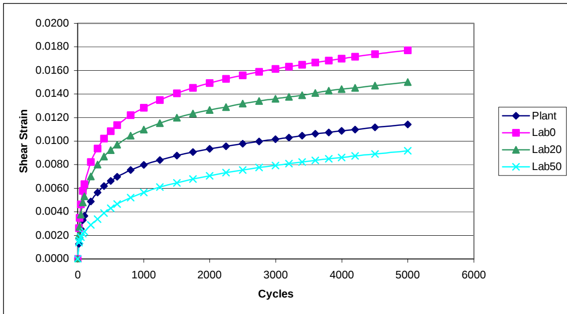
Figure 26 Average Shear Strain from RSCH Test, Missouri Mixes
