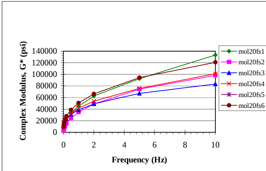
Figure 6 Frequency Sweep Results for Missouri Lab Mix Replicates, 20% RAP (40°C)
