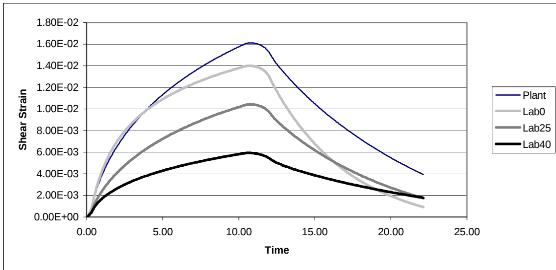
Figure 21 Average Shear Strains for Michigan Mixes at 40°C
