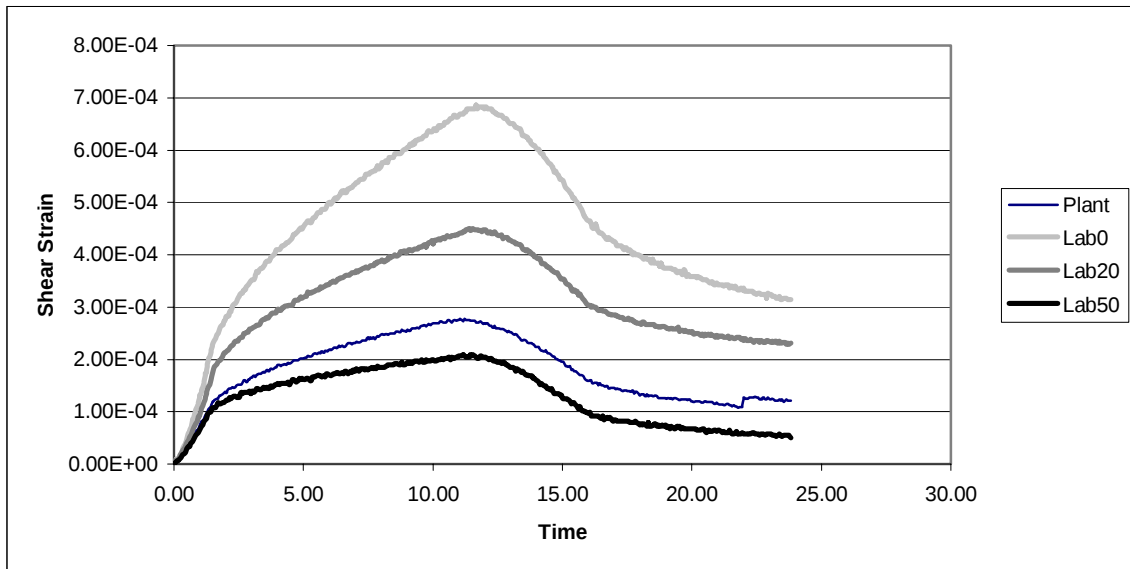
Figure 22 Average Shear Strains for Missouri Mixes at 20°C
