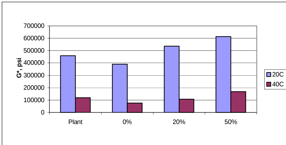
Figure 16 Summary of Complex Shear Moduli from Frequency Sweep at 10 Hz, Missouri
