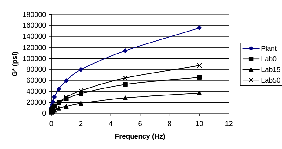
Figure 9 Average Frequency Sweep Results for Indiana Mixes (40°C)
