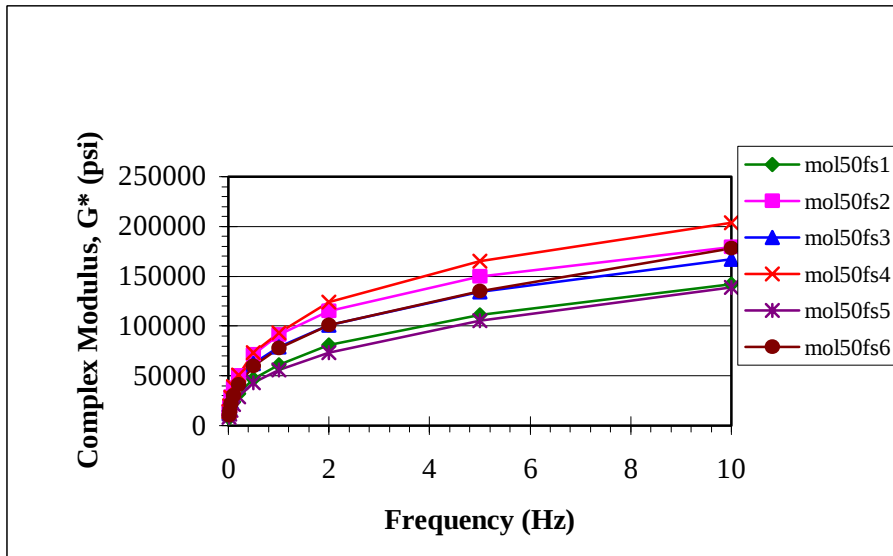
Figure 7 Frequency Sweep Results for Missouri Lab Mix Replicates, 50% RAP (40°C)
