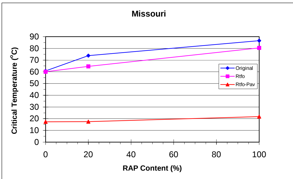
Figure 3 Critical Temperatures vs. RAP Content - Missouri
