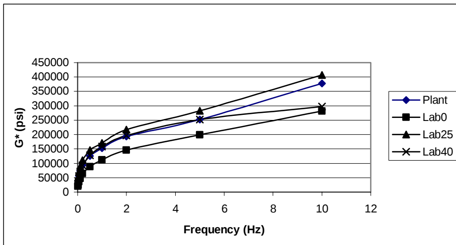
Figure 11 Average Frequency Sweep Results for Michigan Mixes (20°C)
