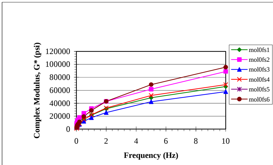
Figure 5 Frequency Sweep Results for Missouri Lab Mix Replicates, 0% RAP (40°C)
