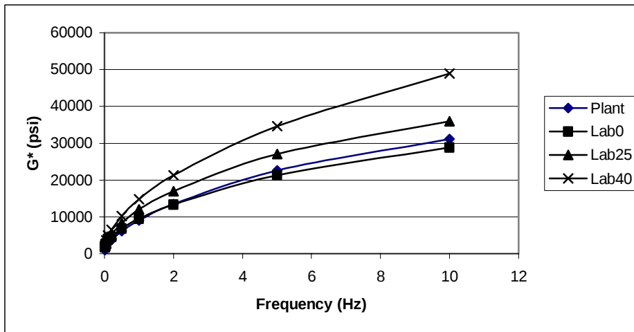
Figure 12 Average Frequency Sweep Results for Michigan Mixes (40°C)
