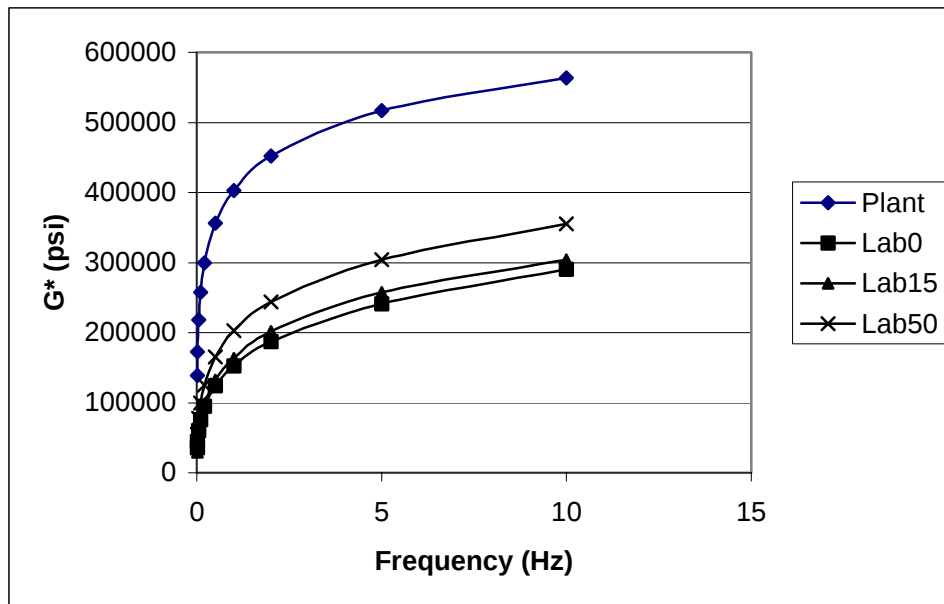
Figure 8 Average Frequency Sweep Results for Indiana Mixes (20°C)
