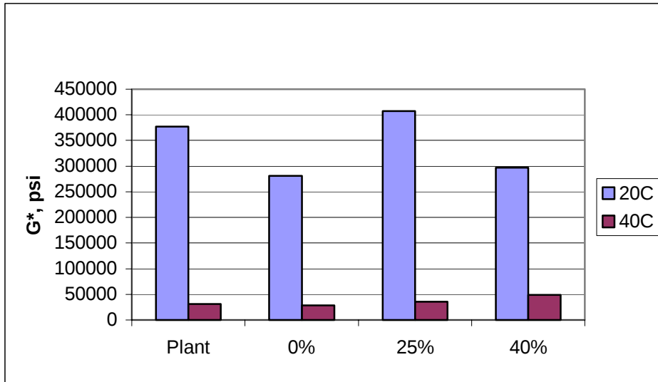
Figure 13 Summary of Complex Shear Moduli from Frequency Sweep at 10 Hz, Michigan
