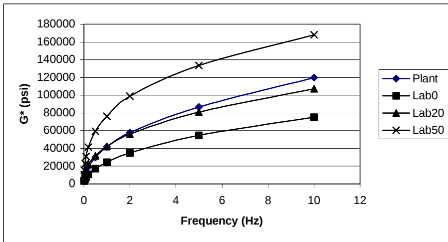
Figure 15 Average Frequency Sweep Results for Missouri Mixes (40°C)
