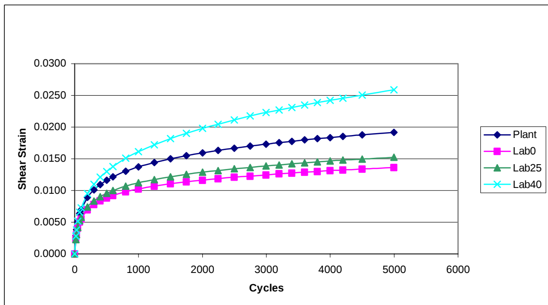
Figure 25 Average Shear Strain from RSCH Test, Michigan Mixes
