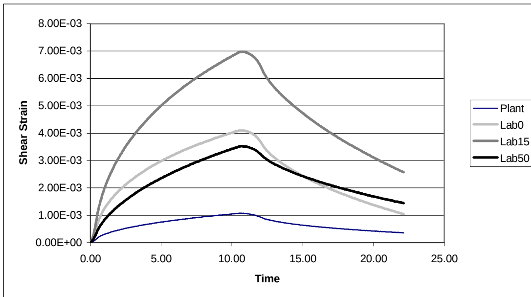
Figure 18 Average Shear Strains for Indiana Mixes at 40°C
