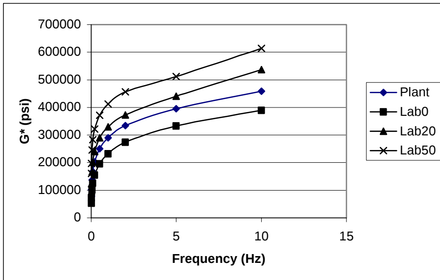
Figure 14 Average Frequency Sweep Results for Missouri Mixes (20°C)
