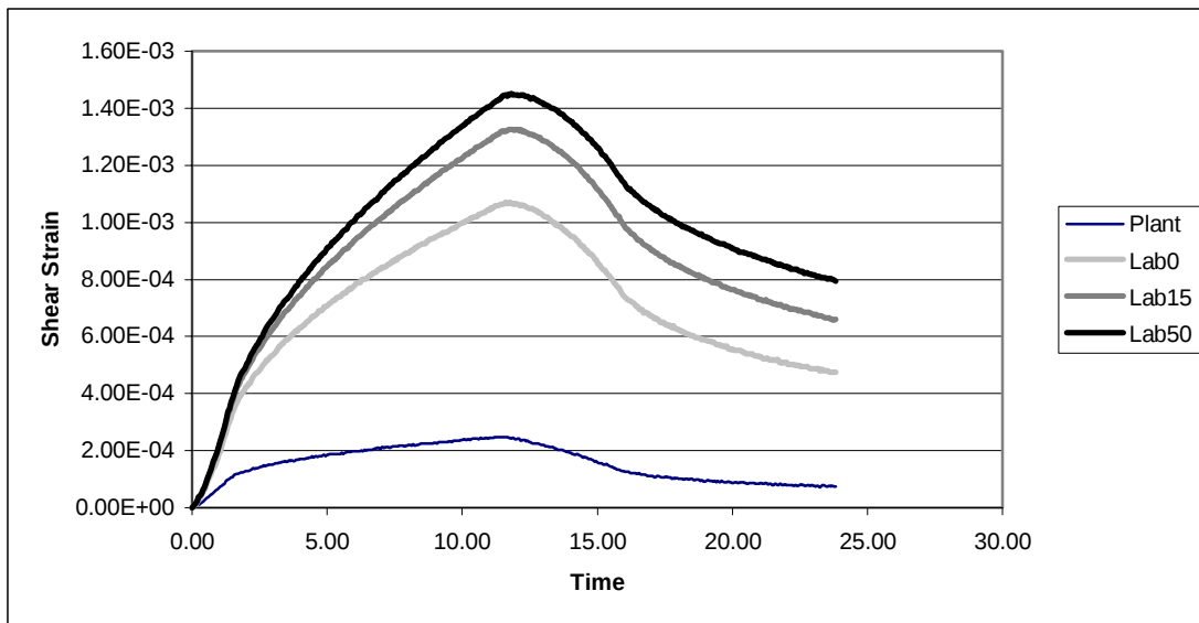
Figure 17 Average Shear Strains for Indiana Mixes at 20°C
